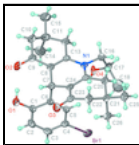
Fig. 1. Thermal ellipsoid plot (Barbour, 2001) of C_{26}H_{32}BrNO_4 at the 70% probability level; hydrogen atoms are drawn as spheres of arbitrary radius. The disorder is not shown.
